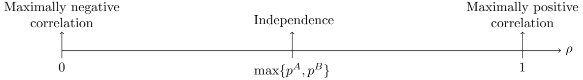
Figure 1: Parametrization of the correlation between the unit A and B's t = 2 payoffs conditional on the units' asset success probabilities at t = 1 .
