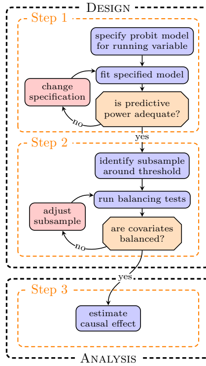
Figure 1: Three-step estimation procedure for causal estimand
