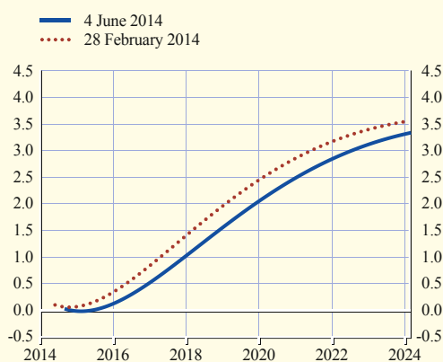
Chart 25 Implied forward euro area overnight interest rates
