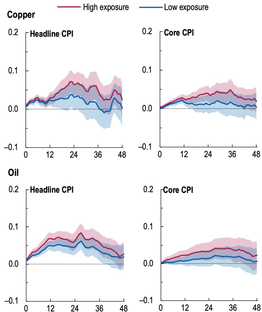
Figure C.4: Impulse Response Functions Taking Heterogeneity in the Net Import Share of Metals and Oil Into Account.
