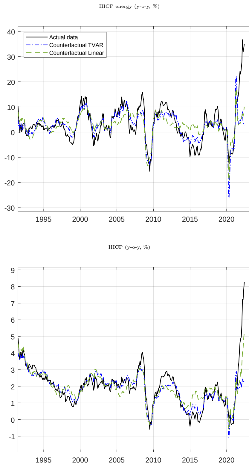
Figure 9: Counterfactual without the Estimated Energy Supply Shocks
