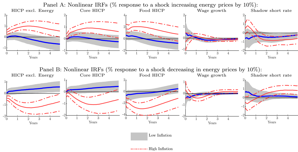
Figure 8: Responses of Prices, Wages and Shadow Short Rate to Energy Supply Shocks
