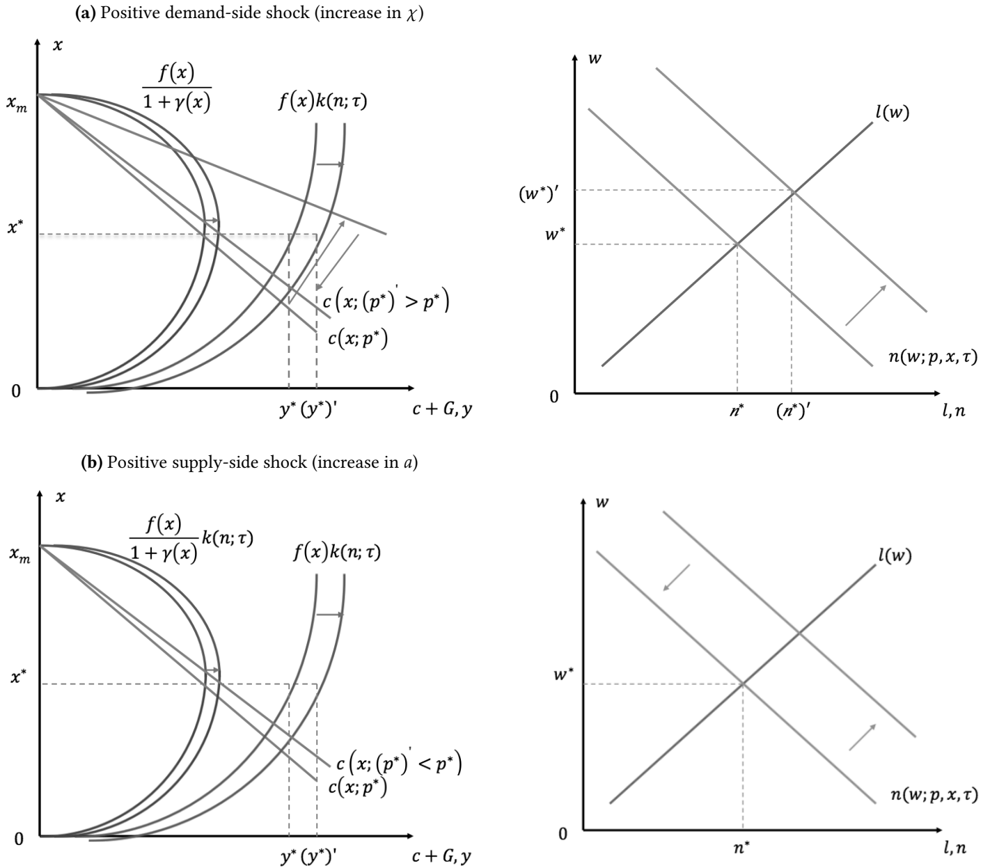
Figure 11: Comparative statics in a competitive equilibrium
