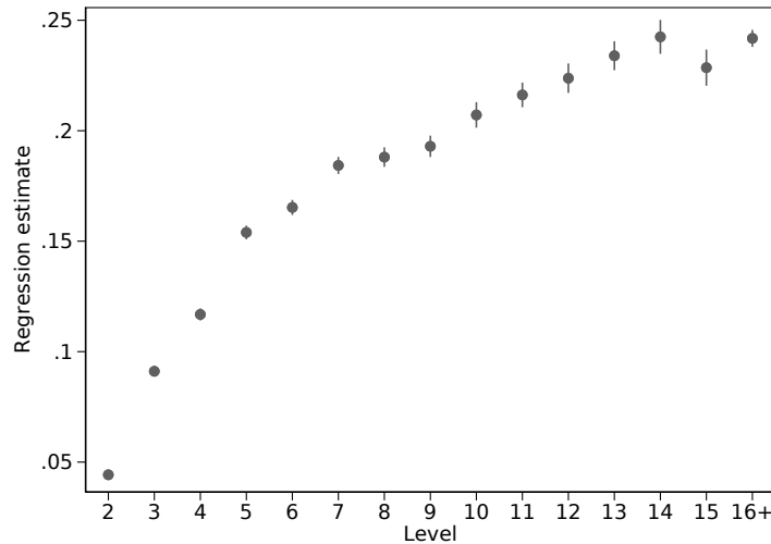
Figure 9: Mincer Regression.
