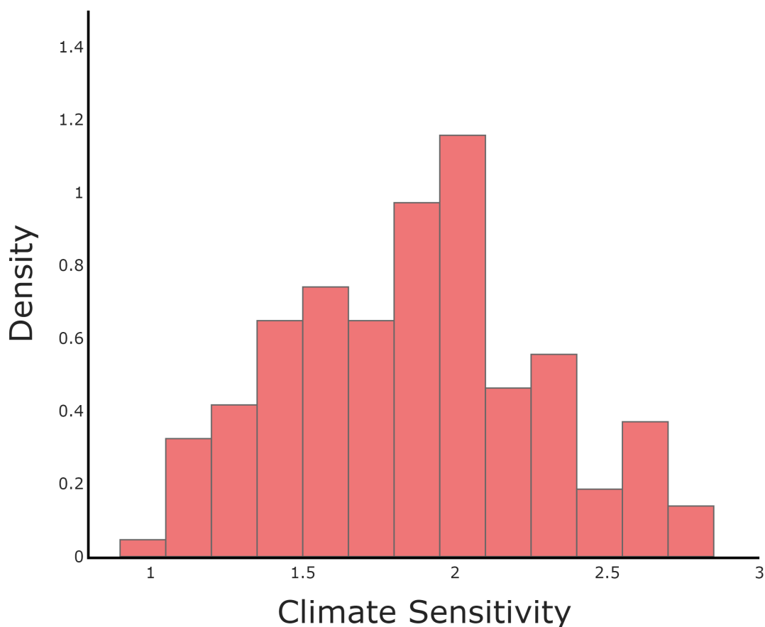
Figure 2: Histograms for the exponentially weighted average responses of temperature to an emissions impulse from 144 different models using a discount rate of one percent.
