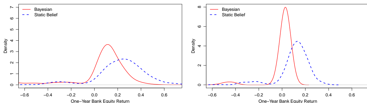
(a) Static Belief v.s. Bayesian: Low Bank Credit
