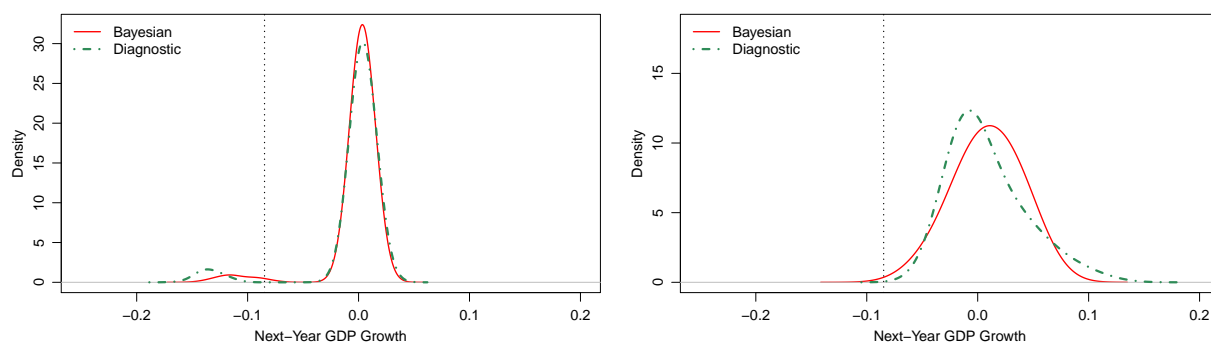
(c) Bayesian v.s. Diagnostic: Low Credit Spread
