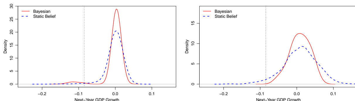
(a) Static Belief v.s. Bayesian: Low Credit Spread
