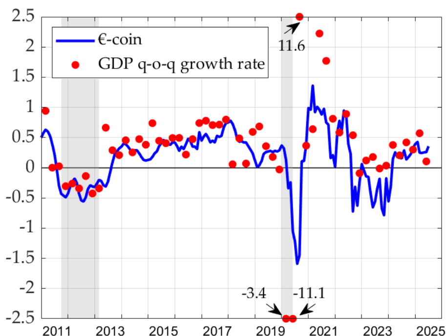
€-coin and euro-area GDP
