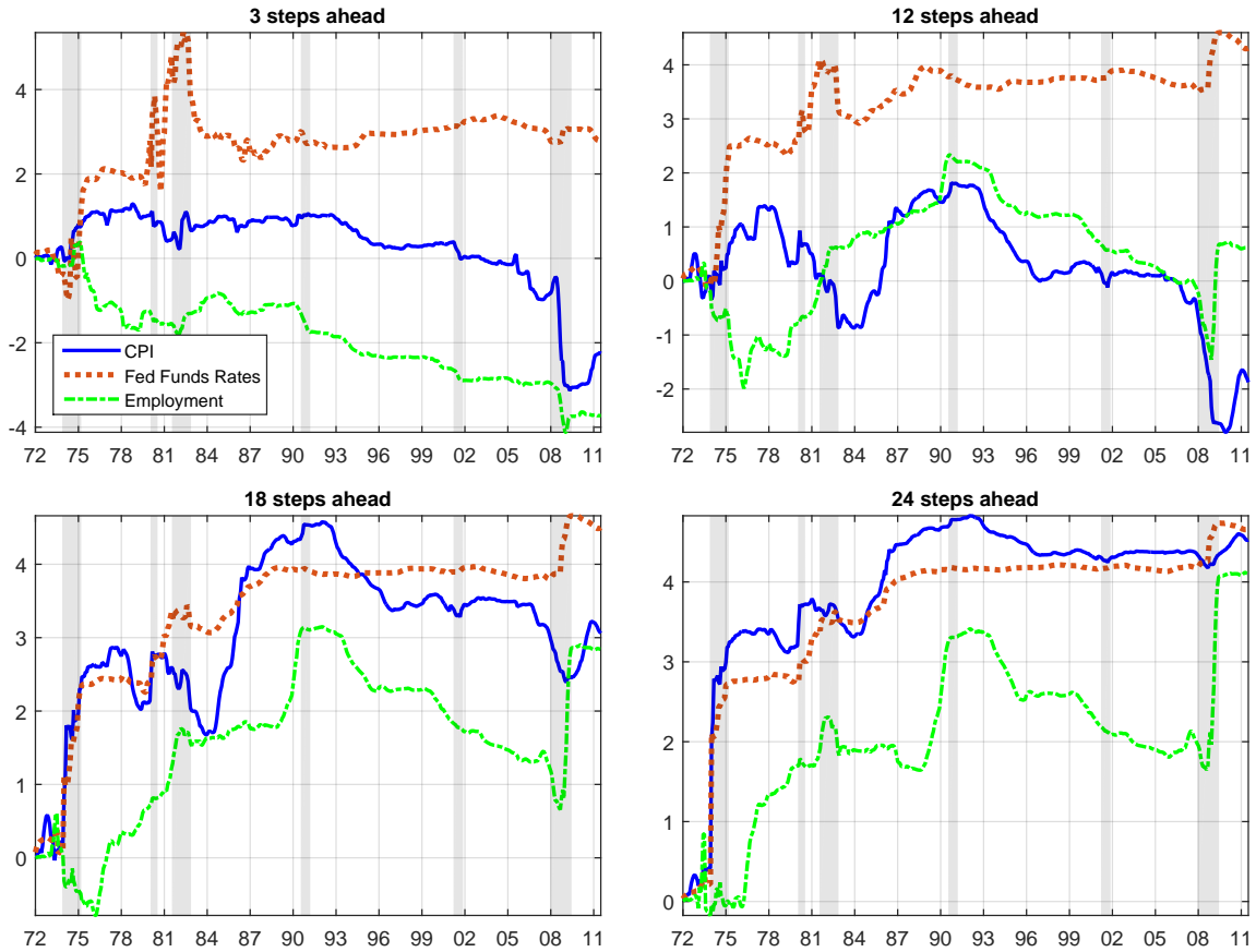
Figure 8: Cumulative sum of squared forecast error differentials: 20 variables combined TVP-VARs versus 78 variables combined TVP-VARs. The figure shows the Cumulative Sum of Squared Forecast Errors Differentials between the equal weights forecast combination of 20 variables VARs with time varying parameters and equal weights forecast combination of 78 variables VARs with time varying parameters. Positive and increasing values indicate that the TVP model with 20 variables outperforms the benchmark, while negative and decreasing values suggest the opposite. Shaded areas indicated NBER-dated recessions.
