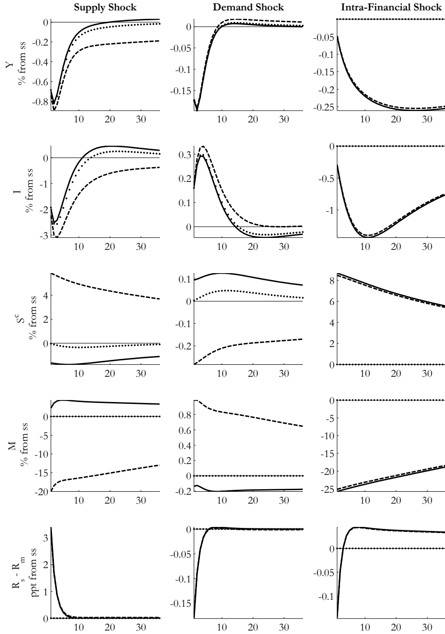
Figure 4: Impulse response functions
