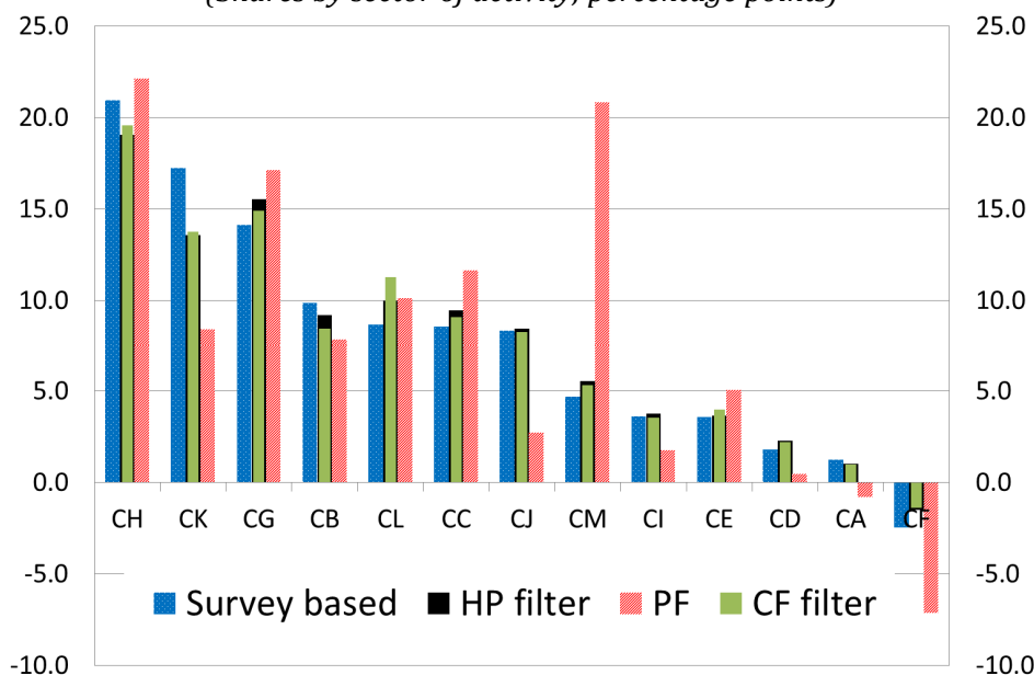
Baseline contributions to capacity loss by activity sector (Shares by sector of activity; percentage points)
