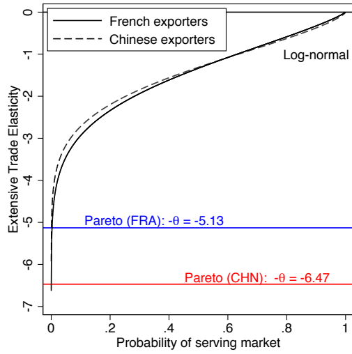
(a) theory
