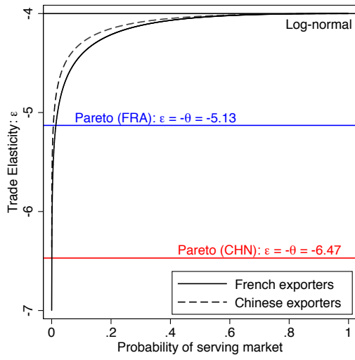
(a) theory
