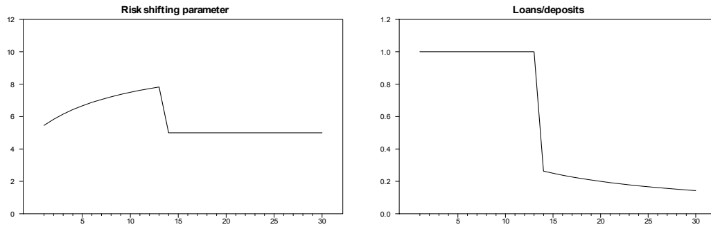
Fig. 4. CVH model (A=0.1, beta=5, r =1.1)
